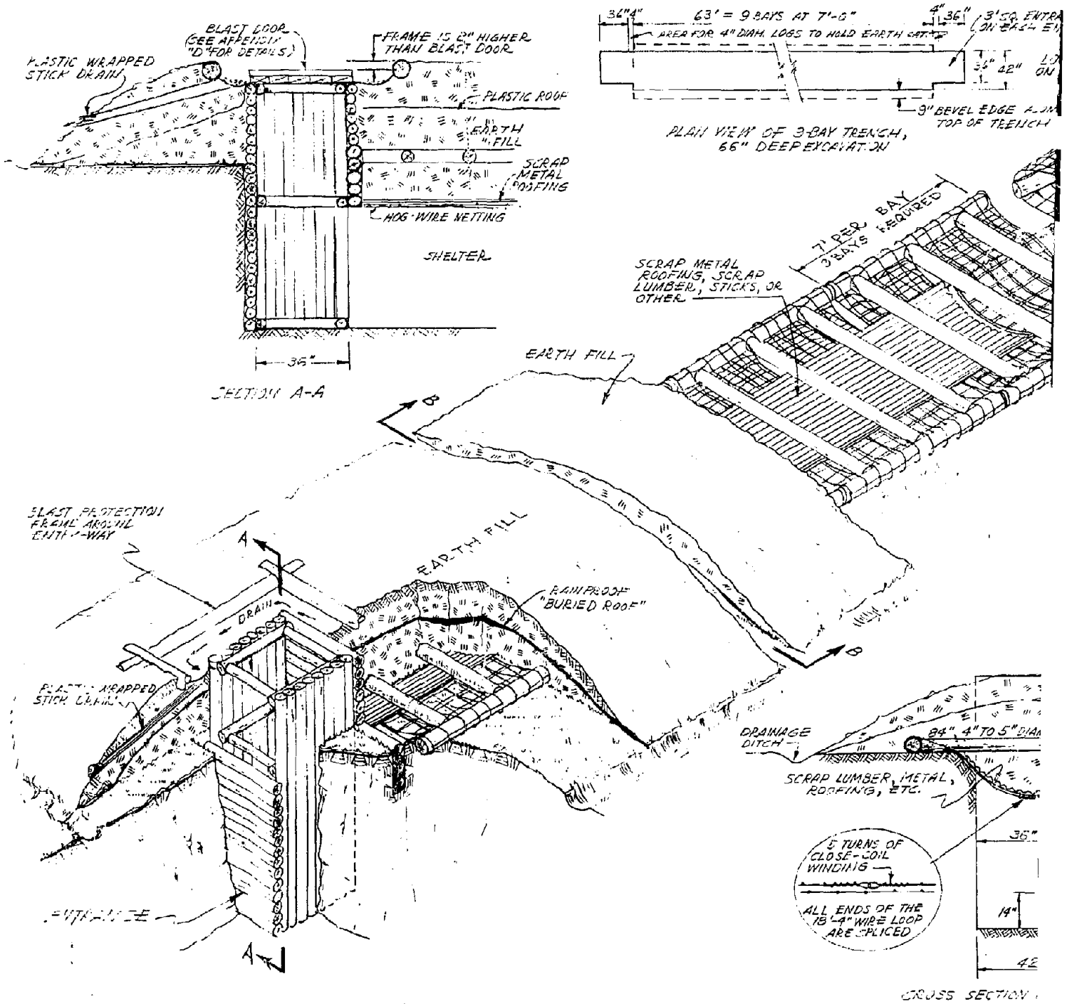
Fig. A-3.2. Catenary wire roofed shelter - alternate design.
